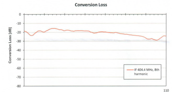
Figure 3 THZWHM-10P Conversion Loss
