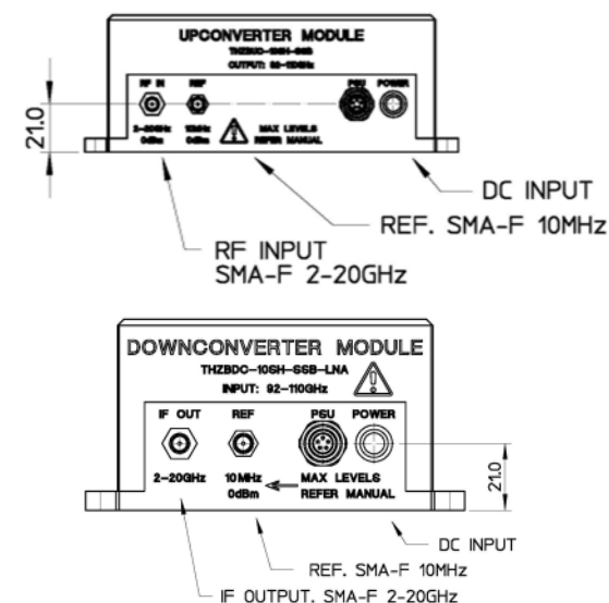
Fig 2 Converter Interfaces
