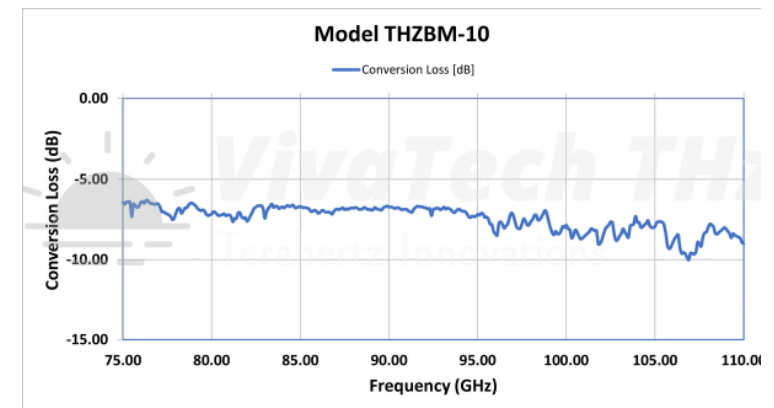
Figure 1 Full Band Fundamental Balanced Mixers
