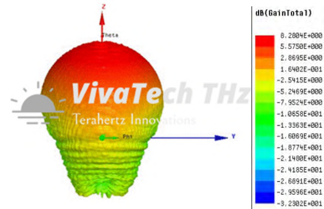
Beam Pattern THZWGP-03-50
