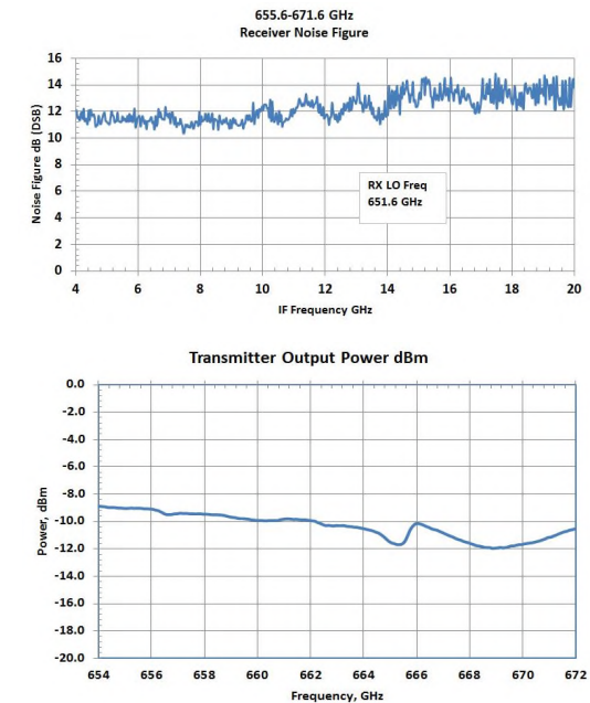
Fig 2 Noise Figure / Output Power
