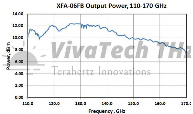
Figure 2 THZXFA-06FB Output Power
