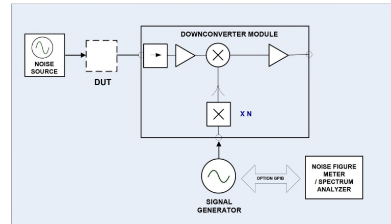
Figure 2. Noise Test Set Measurement System
