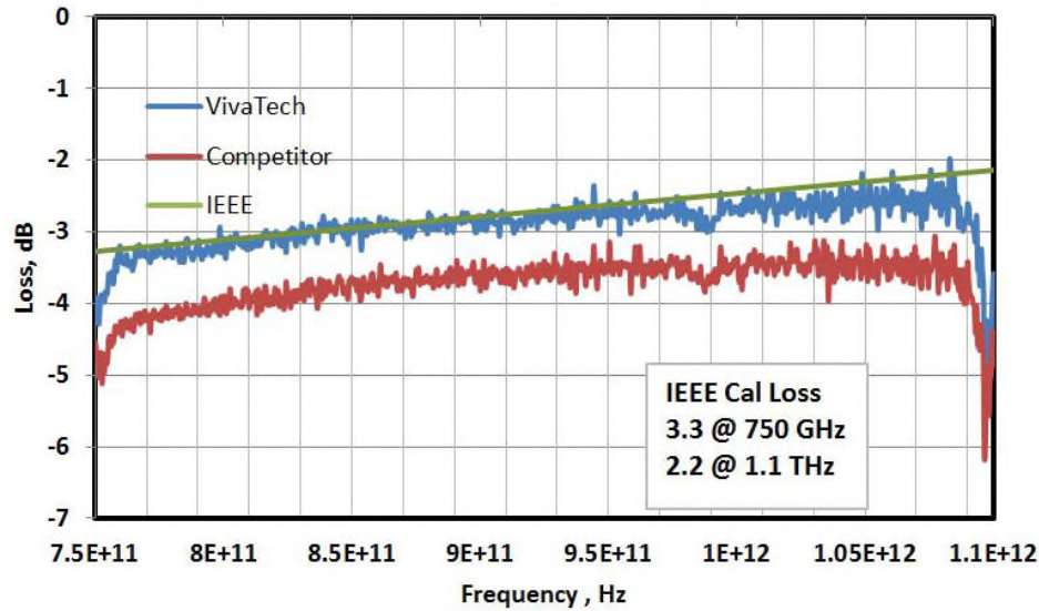
Fig 1 Loss comparisons & IEEE waveguide standard 750-1100 GHz
