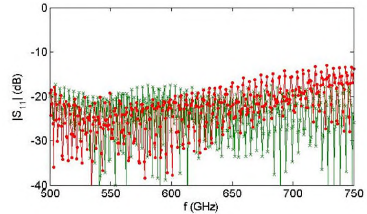
Fig 2 WR1.5 500-750 GHz Return Loss, 25/50 mm lengths
