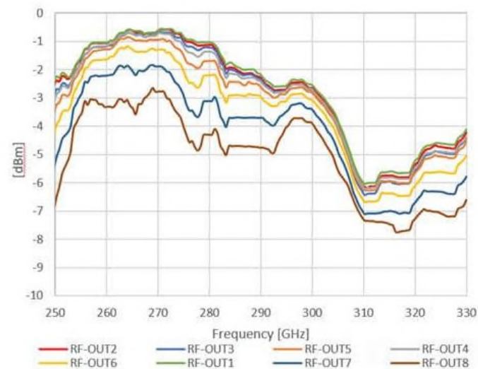
Figure 3 Gain Compression
