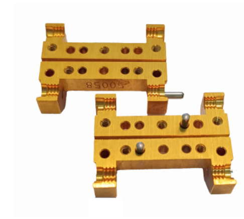
Figure 2 THZWGTA-10-12 internal
