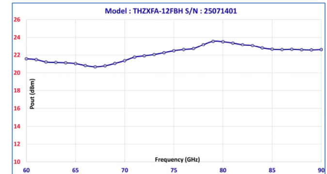
Figure 2 THZXFA-12FBH Output Power
