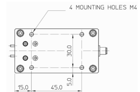
Figure 2 Model THZW HM-10P (DC port not shown)
