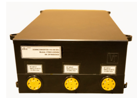
Fig 2 110-330 GHz Downconverter
