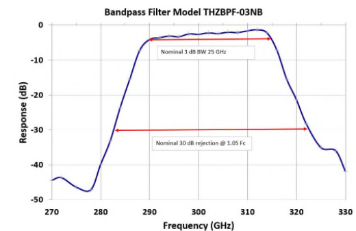
Figure 2 THZBPF-03 290-310 GHz
