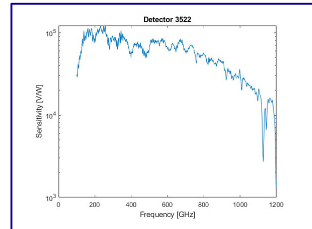
Figure 2 THZWDM-WB Typical Sensitivity
