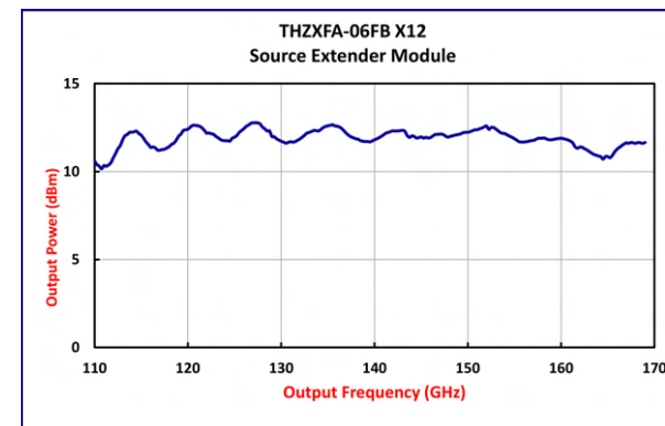
Figure 2 THZXFA-06FB Output Power
