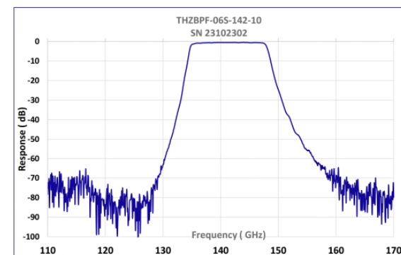
Figure 2 THZBPF-06 135-145 GHz
