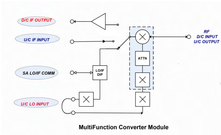
Fig 5 : Functional Schematic
