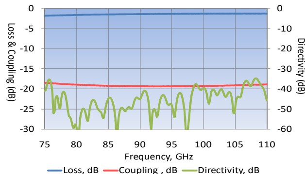
W Band 3 port 20 dB Coupler Typical Performance
